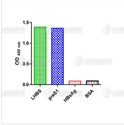
Direct ELISA of HBV preS1 antibody, clone S101
